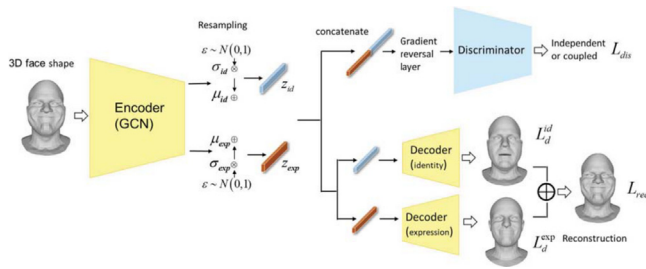
Fig. 6. DI-MeshEncoder structure [2] (courtesy of Prof. Huibin Li).
