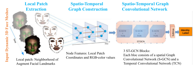
Fig. 16. Overview of the Face-GCN [8].
