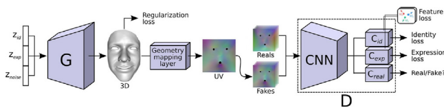
Fig. 10. The methodological structure of the literature [64] (courtesy of Victoria Fernández Abrevaya).
