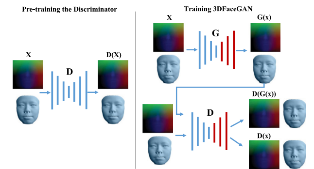
Fig. 11. 3DFaceGAN network structure [65].
