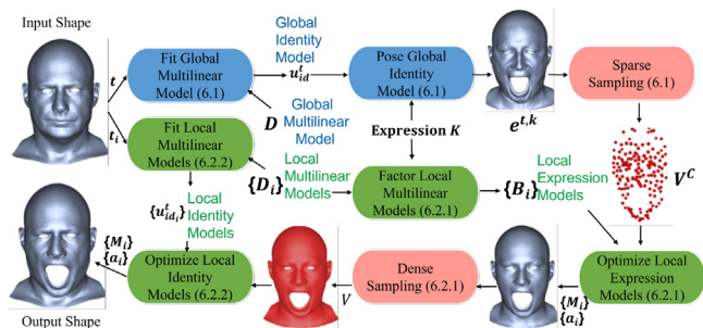
Fig. 12. Global-local multilinear model framework [66].
